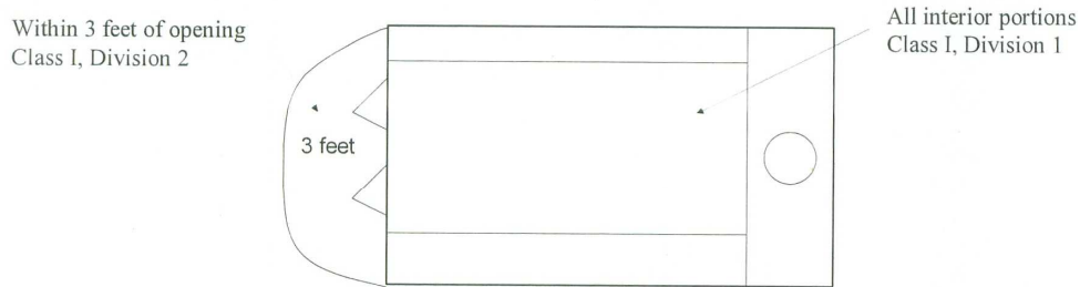
Typical Enclosed Vehicle Spray Booth (plan view)
